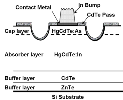
Figure 2. Buffer layers mediate the lattice spacing mismatch.
