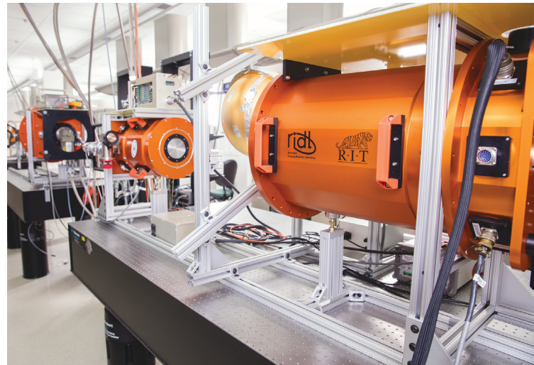
Imaging Detector Testbeds: These high-performance imaging detector testbeds in RIT's Center for Detectors give the FPI unique abilities to develop imaging devices for use in NASA missions.
